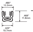
1318-1951-0 .080" pile, w/.030" galvanized wire 1334-2061-8 .080" pile, w/.032" aluminum wire 1379-2601-9 .100" pile, w/.032" aluminum wire
