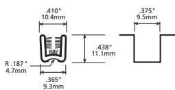
1318-1951-0 .080" pile, w/.030" galvanized wire 1334-2061-8 .080" pile, w/.032" aluminum wire 1379-2601-9 .100" pile, w/.032" aluminum wire
