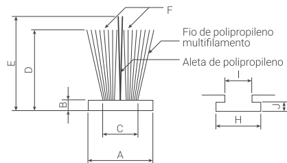
FIN-SEAL (FS)
