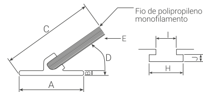
ANGLE-PILE (AP)
