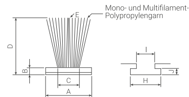
SHUTTER PILE (SP)
