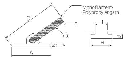
ANGLE-PILE (AP)
