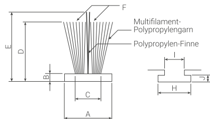
FIN-SEAL (FS)
