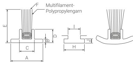
POWER-PILE (PW)
