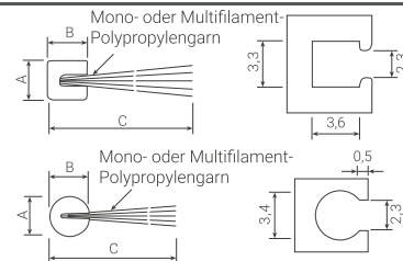
SKIRTING-FRIDGE (SF)
