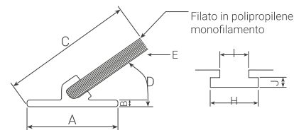
ANGLE-PILE (AP)
