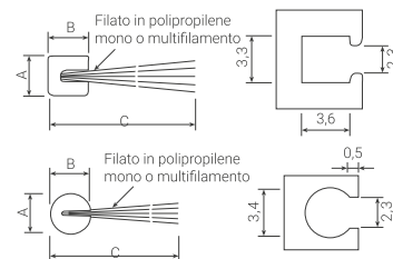
SKIRTING-FRIDGE (SF)
